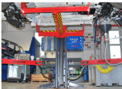
Easy access to vehicles un- derside due to H-design of the carriage
